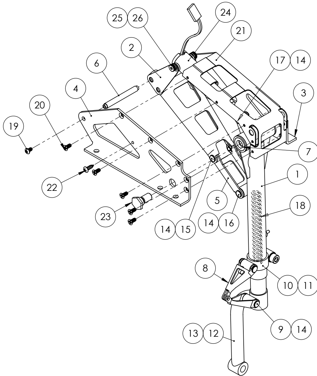
AXLE BAG ASSEMBLY - #145142A
