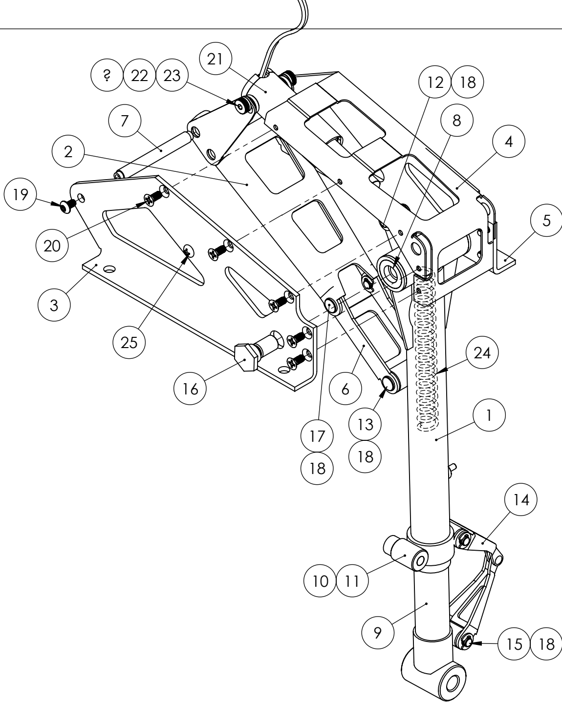
AXLE BAG ASSEMBLY - #145142A
