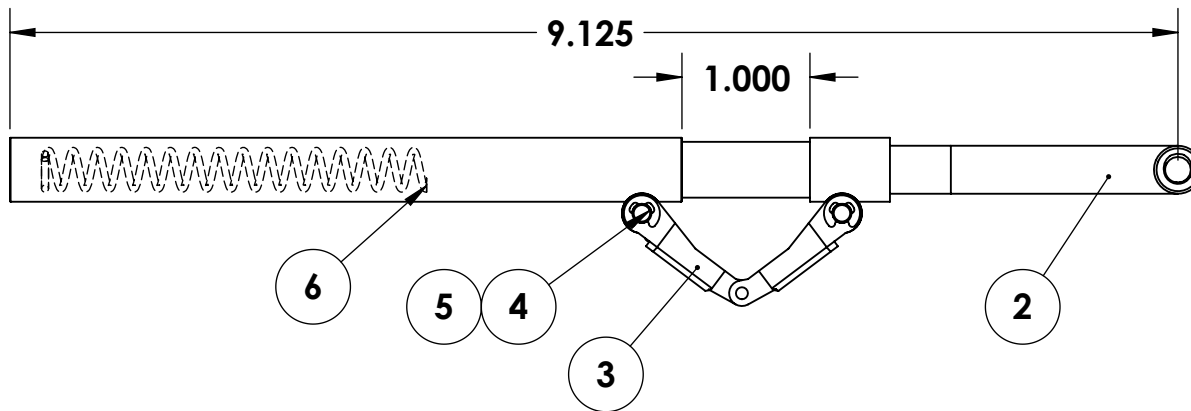
AXLE BAG ASSEMBLY - #671142A
