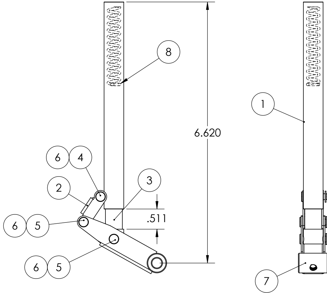
AXLE BAG ASSEMBLY - #670142A
