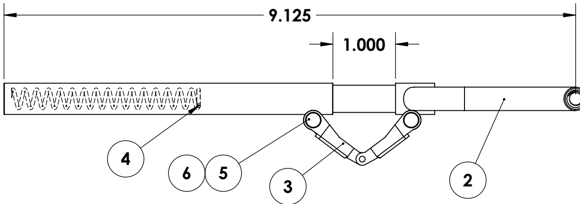
AXLE BAG ASSEMBLY - #671142A
