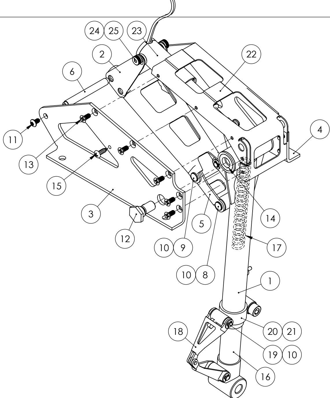
AXLE BAG ASSEMBLY - #145142A
